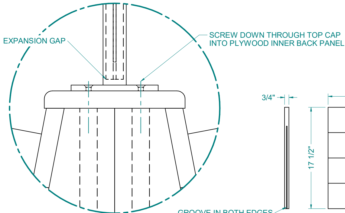
DETAIL A
